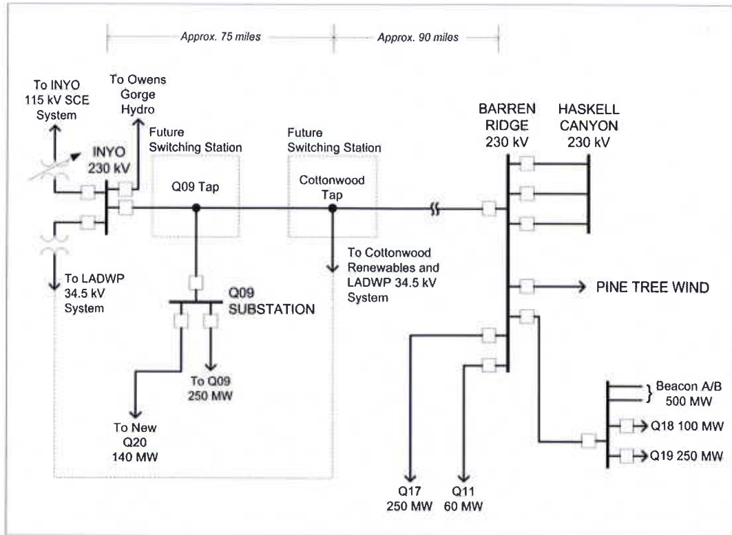
Figure 5-1 – Barren Ridge – Inyo Path Connection Detail
