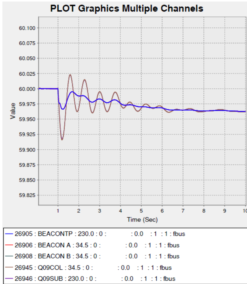
Figure 2-9 Trip Beacon – Frequency Plots, Value=Hz
