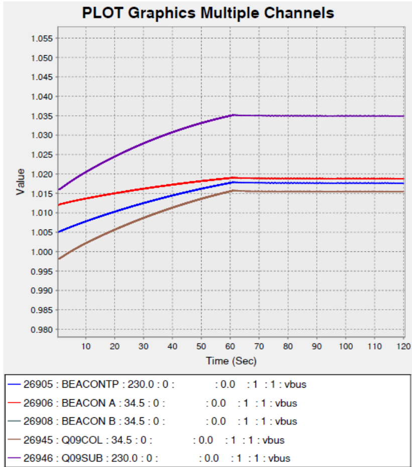
Figure 2-8 50% Ramp Over 1 Minute – Voltage Plots, Value=per-unit
