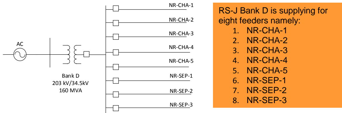
Figure ES 2: One line diagram - LADWP circuit supplied by RS-J Bank D
