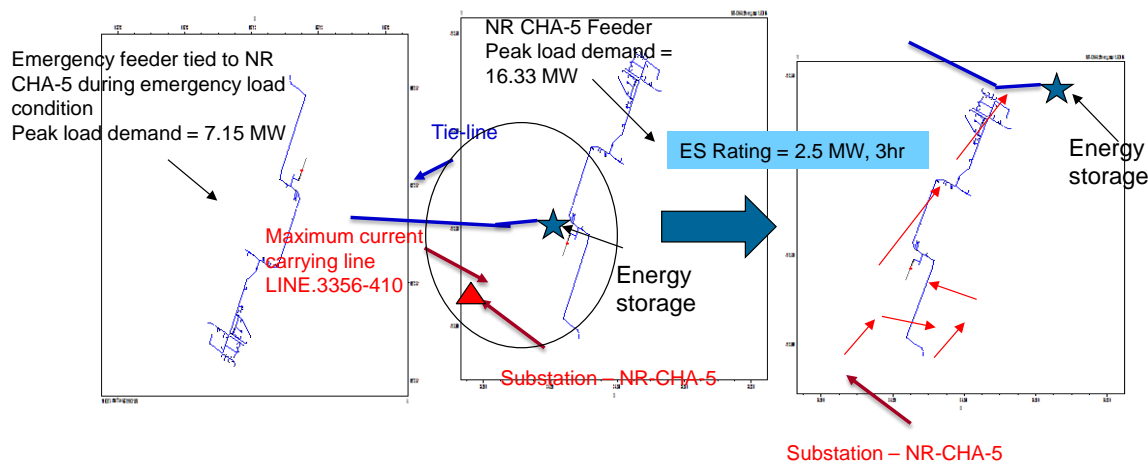
Figure ES 5. Energy Storage to Avoid Distribution Line Overloads under Emergency Load Transfer
