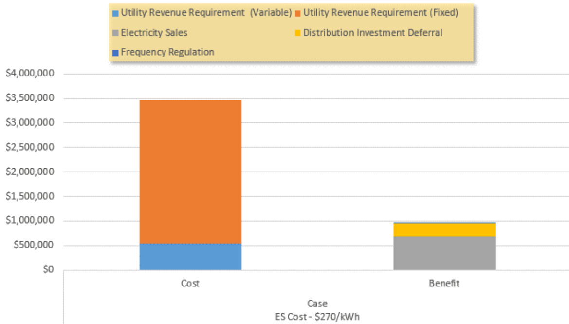
Figure ES 6: Total Cost and Benefit Results for the Stacked Benefit Case
