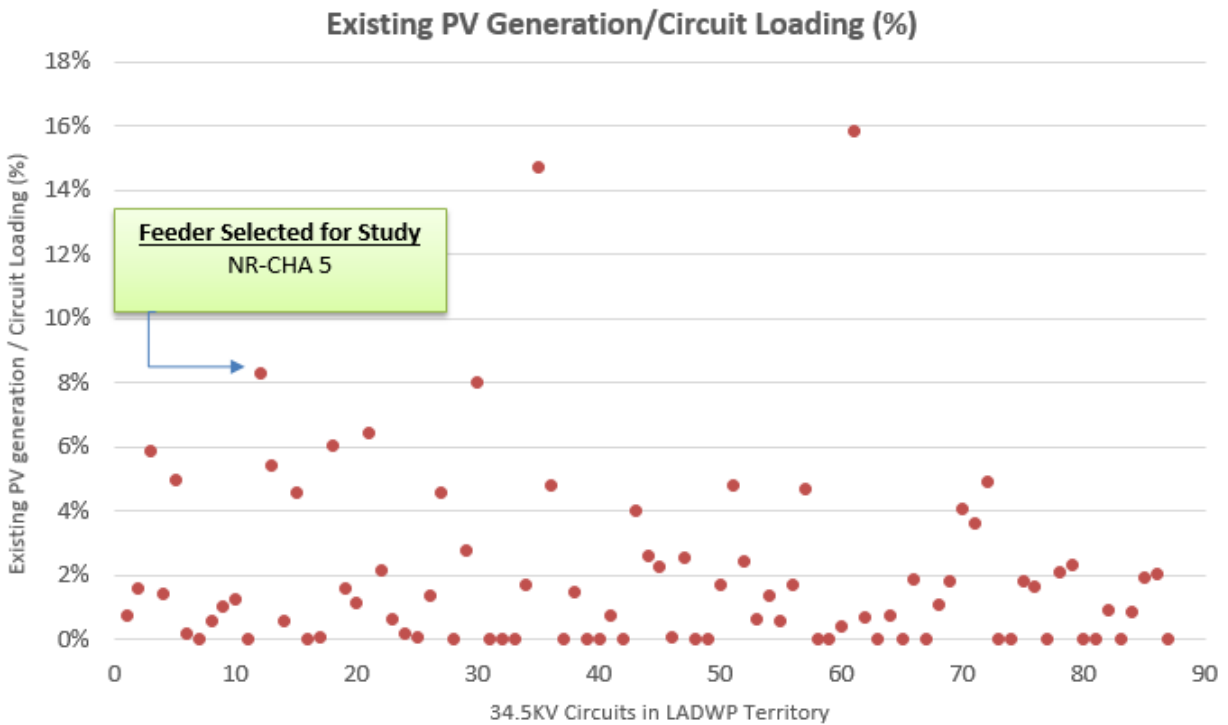
Figure ES 1: LADWP Feeder Loading Characteristics – A Comparison
