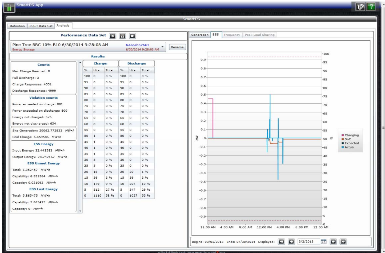
Figure 2-2 SmartES Screenshot of BESS Response from Pine Tree Solar
