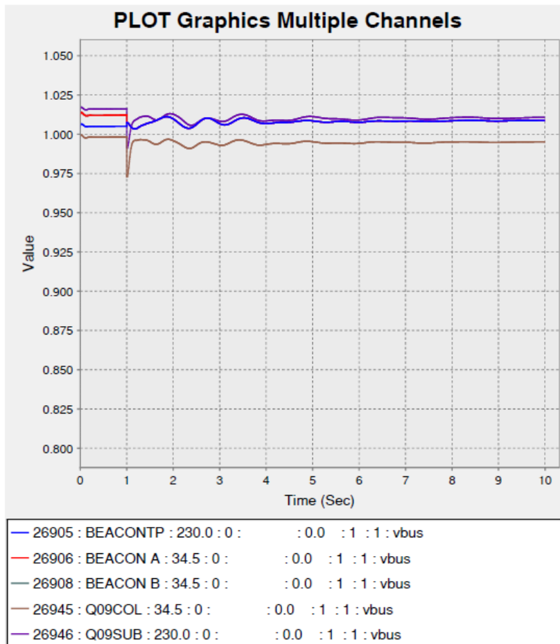
Figure 2-10 Trip Beacon – Voltage Plots, Value=per-unit
