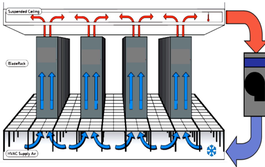
Figure 1: Example of Aisle Containment Using Chimney Racks
