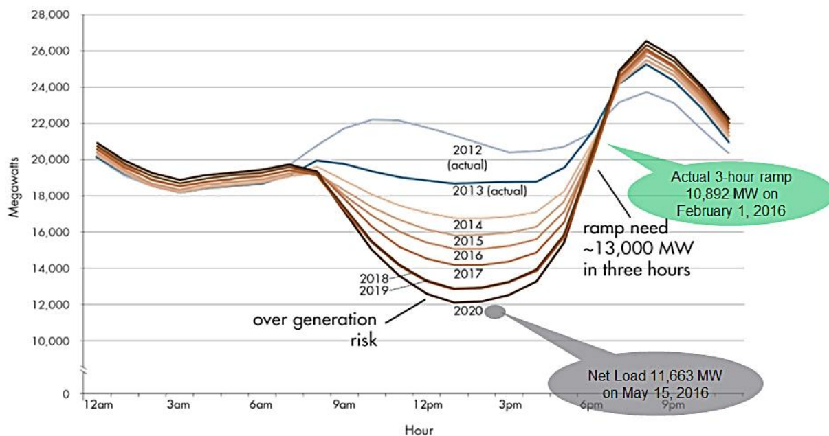
Figure 1: Net Load “Duck Curve” for a Typical Spring Day
