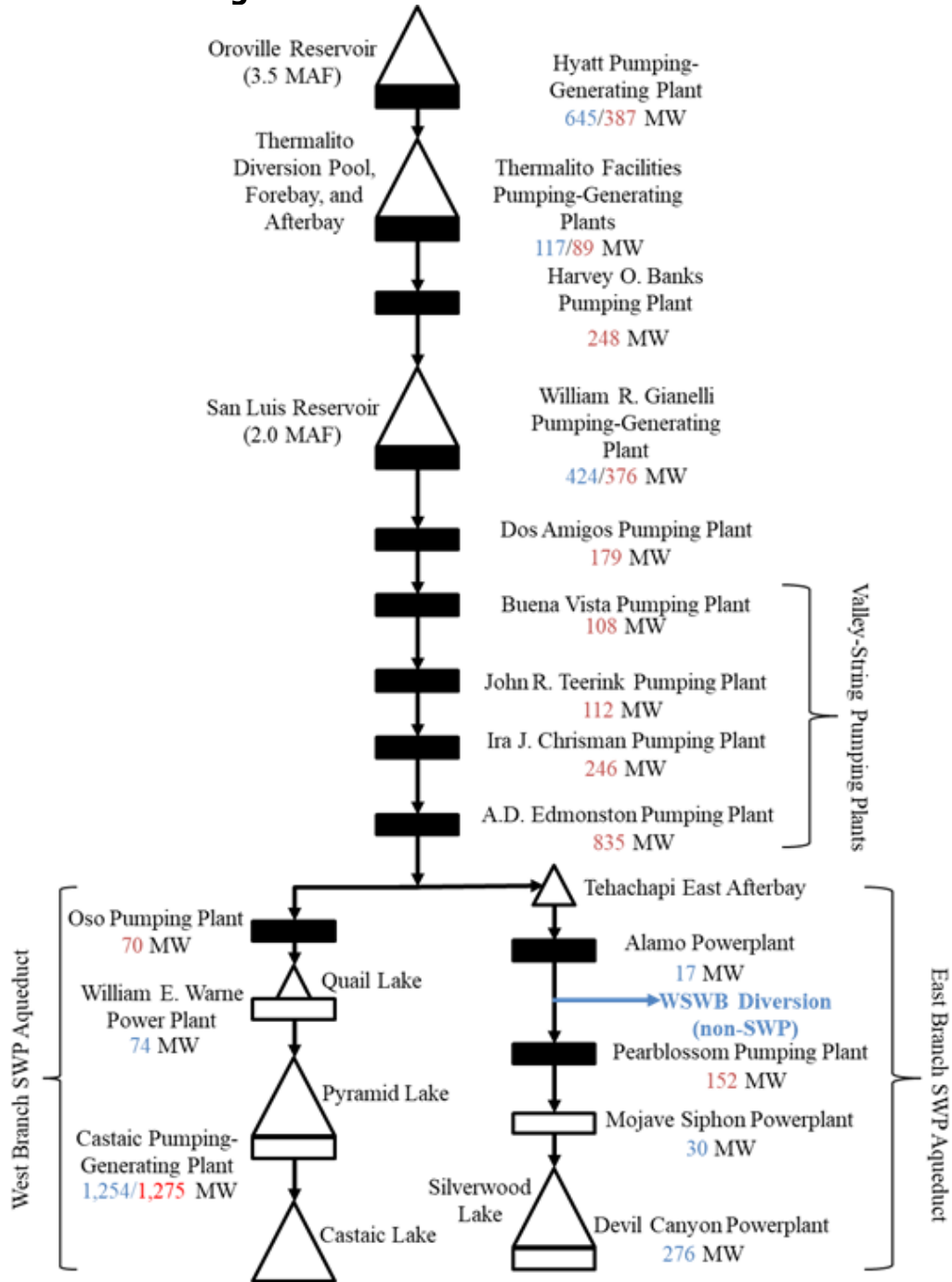
Figure 6: Schematic of SWP Facilities
