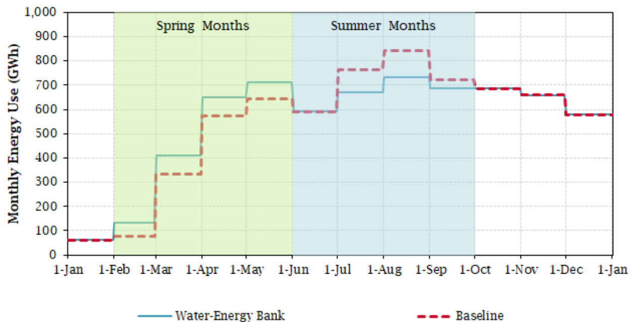
Figure 13: Example Year 1940 Net Energy Use to Convey Water Between San Luis Reservoir and WSWB for the Baseline and Water-Energy Bank Scenarios
