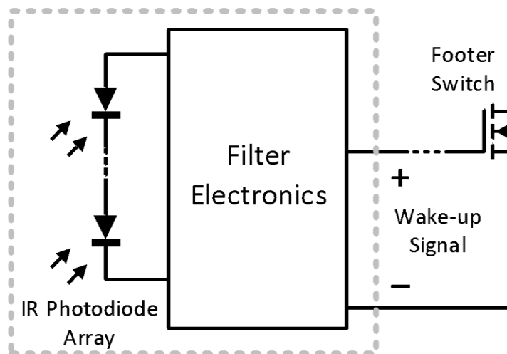
Figure 13: The Receiver for an IR-based Zero-Standby Supply
