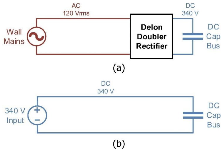
Figure 29: Direct-Direct Current Refrigerator Modification
