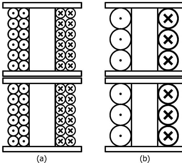
Figure A-1: Winding Area Diagram for Two Motors with Equal Input Power and Magnetic Flux
