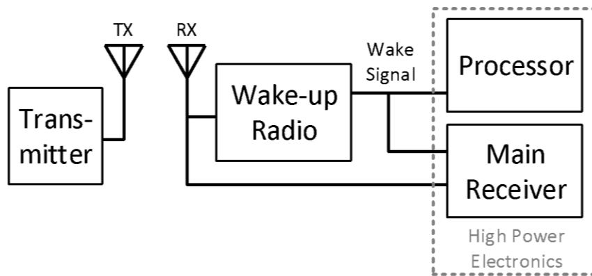
Figure 17: Wake-Up Radio System
