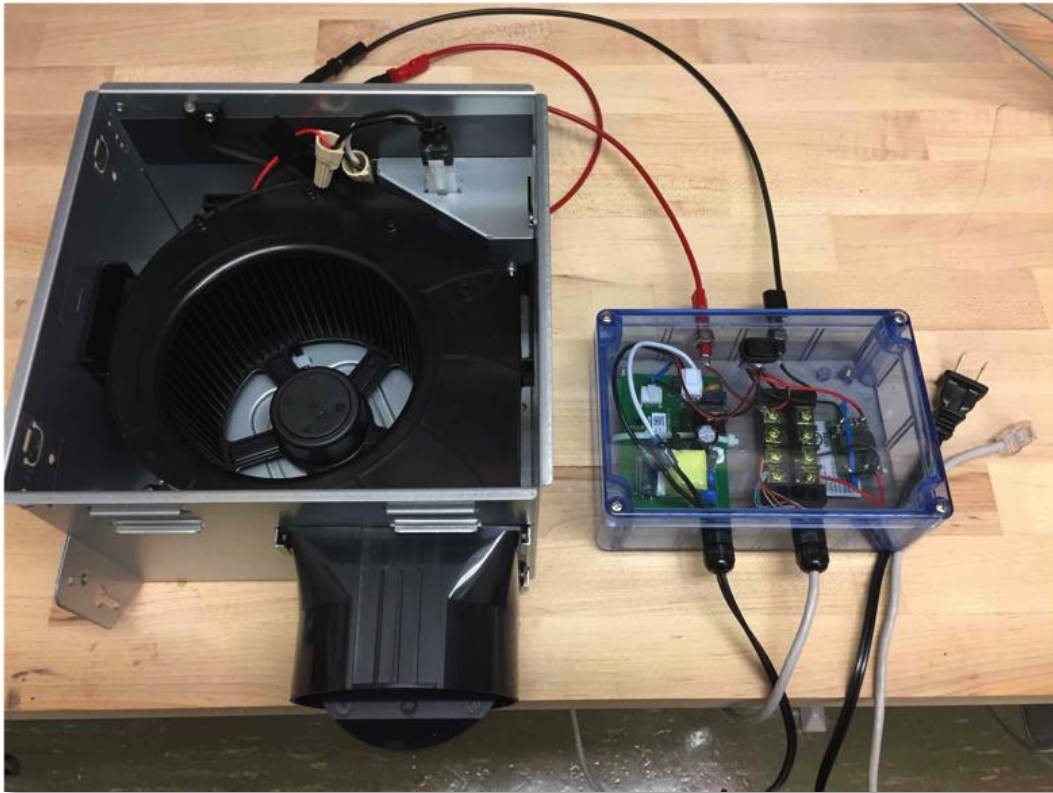
Figure 25: Direct-Direct Current Fan Prototype
