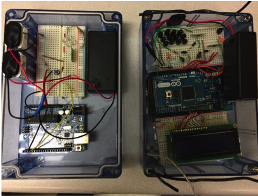
Figure 14: Prototype of the IR-Based Zero-Standby Supply
