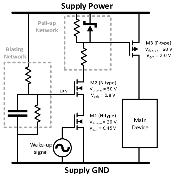
Figure 11: The Cascoded Header Switch
