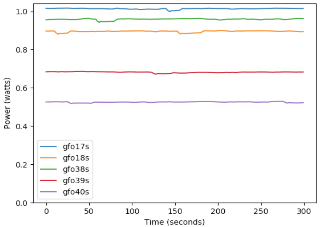
Figure 52: Comparison of Ground Fault Circuit Interrupter Outlet Power
