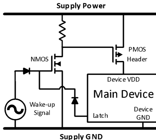
Figure 10: The Header Switch
