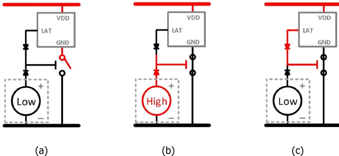
Figure 9: Operation of a Footer Switch
