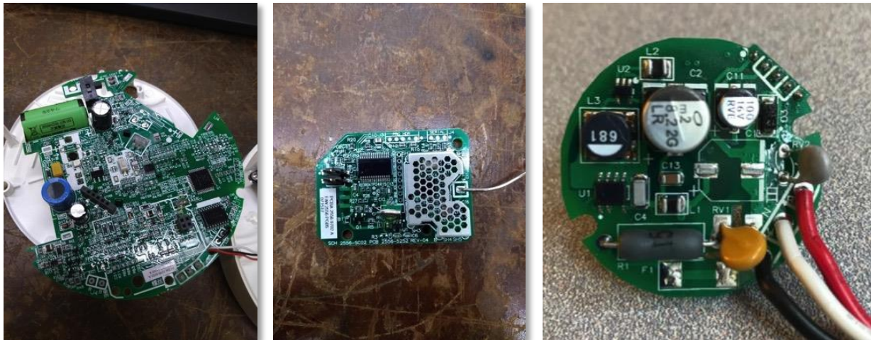
Figure 61: Teardown of the SMA07 Smoke Alarm
