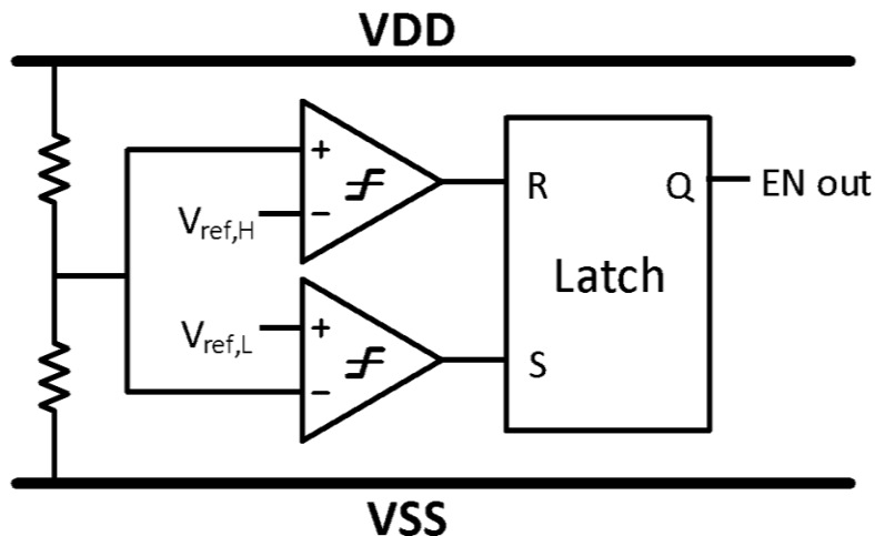
Figure 6: Simple Burst-Mode Logic
