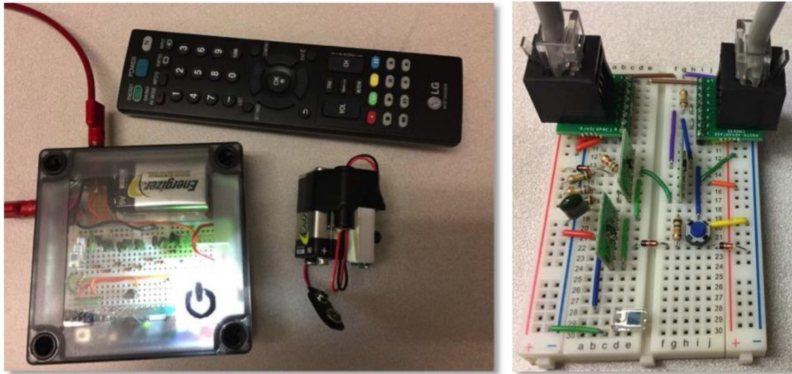
Figure 16: Prototypes of the Laser-Based Zero Standby Supply
