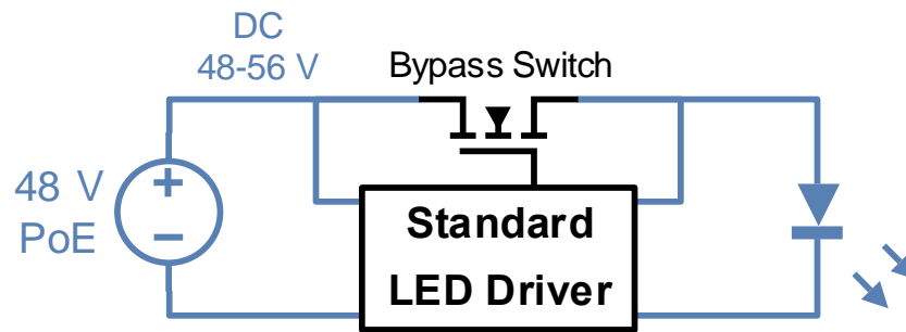
Figure 35: Direct Direct-Current Task Lamp Discussion
