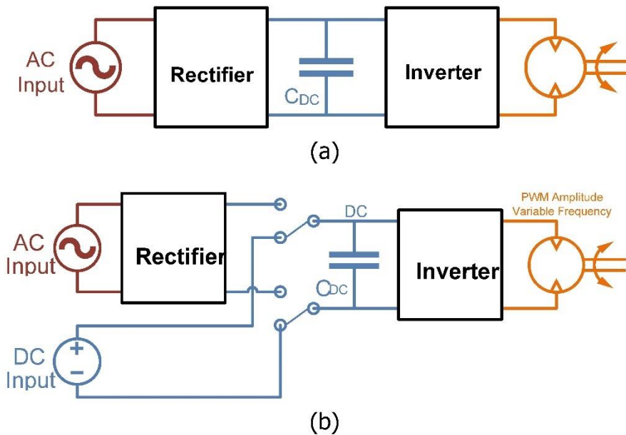
Figure 21: Block Diagram of a Variable Frequency Drive Motor
