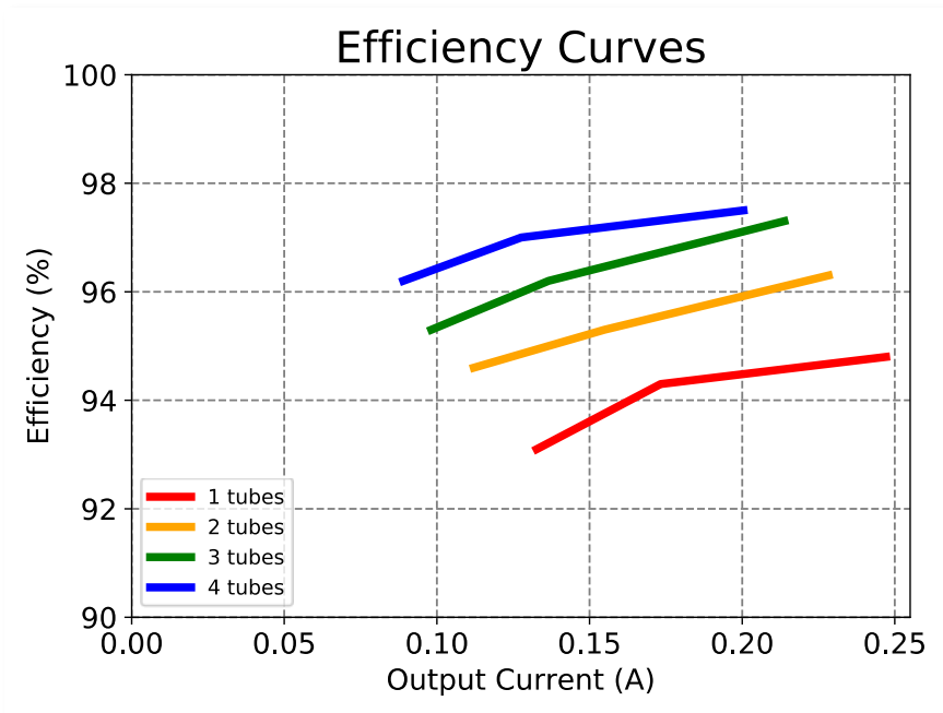
Figure 38: Direct Direct-Current Zone Light Prototype Efficiency
