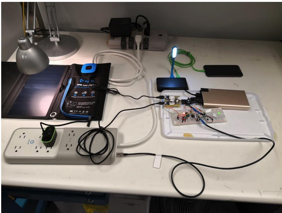
Figure 69: Bench Assembly of a Low-Voltage Residential Direct Current Network with Two Loads
