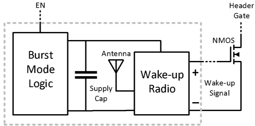
Figure 18: Wake-Up Radio Operational Block Diagram
