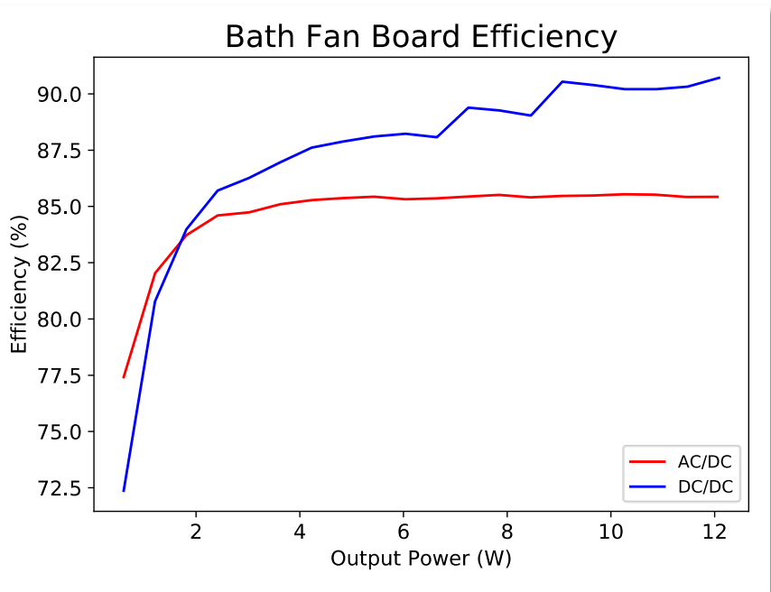
Figure 27: Efficiency Curves for the Bath Fan Boards
