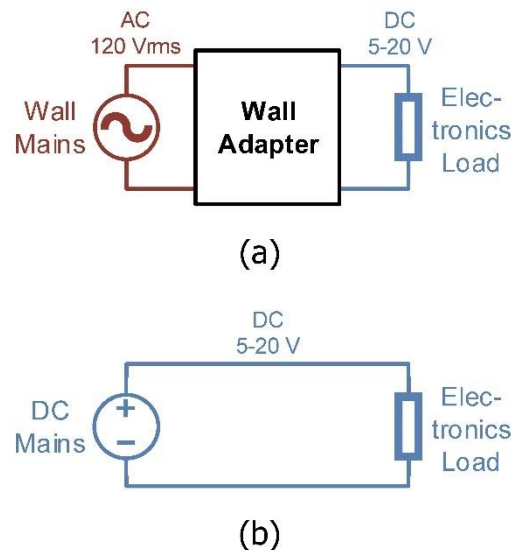
Figure 22: Direct Direct-Current Wall Adapter Modification
