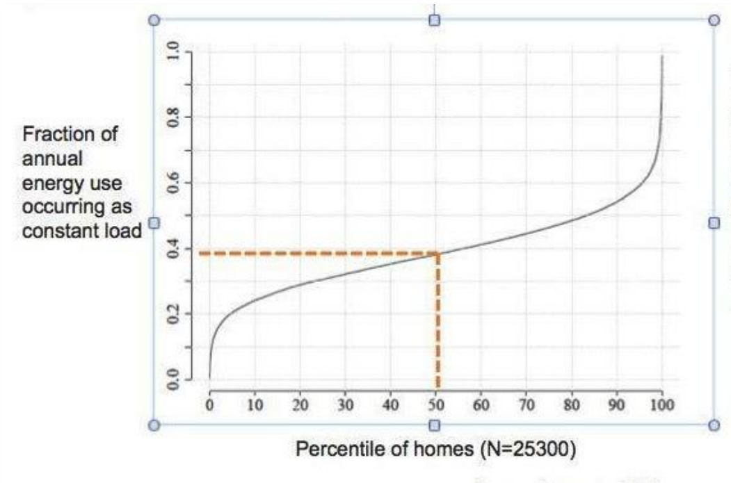
Figure 1: Fraction of Annual Energy Use Occurring as Constant Load
