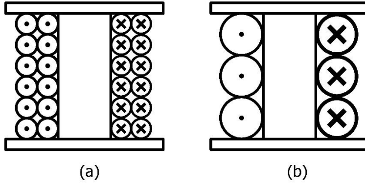
Figure 28: Motor Winding Area
