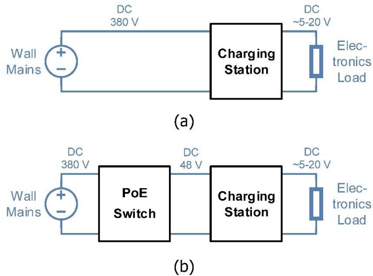
Figure 23: Direct-Direct Current Wall Adapter Discussion
