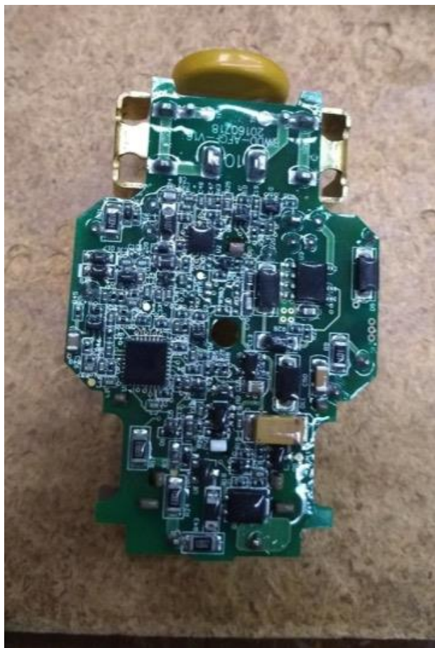
Figure 58: AGO31 AFCI/GFCI Outlet Teardown—Electrical Circuit
