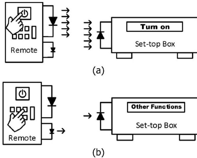
Figure 12: Proposed IR Energy Harvesting Method
