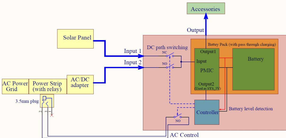
Figure 68: Block Diagram for a Residential Low-Voltage Direct Current Network
