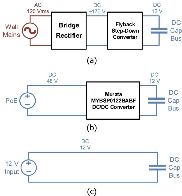
Figure 24: Direct-Direct Current Bath Fan Modification
