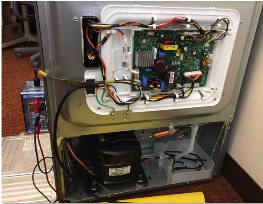
Figure 30: Direct-DC Refrigerator Prototype
