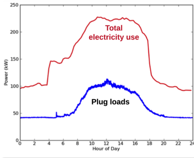
Figure ES-1: Hourly Electricity Use Profiles for Plug Loads and Total Electricity in California Office Building
