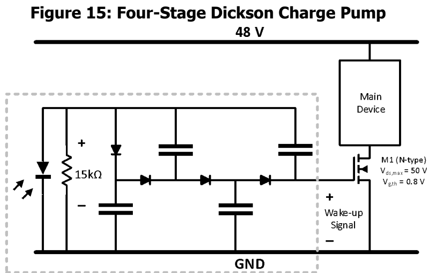
Laser standby solution with a four-stage Dickson charge pump attached to an NMOS footer switch M1.
