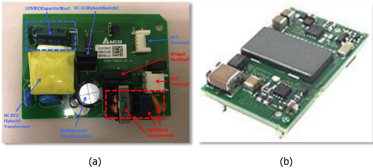
Figure 26: Fan Boards
