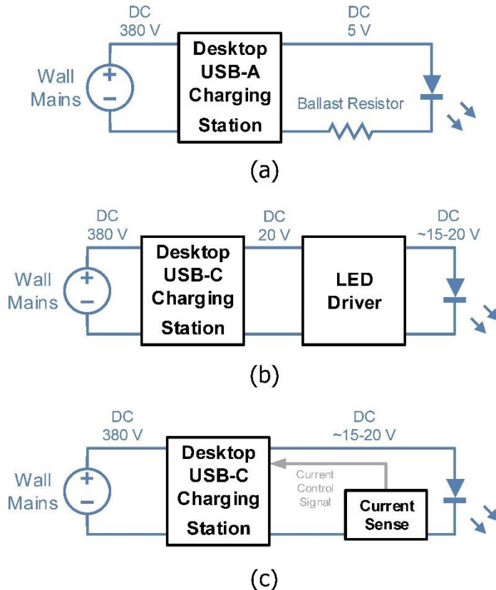
Figure 33: Direct Direct-Current Task Lamp Modification
