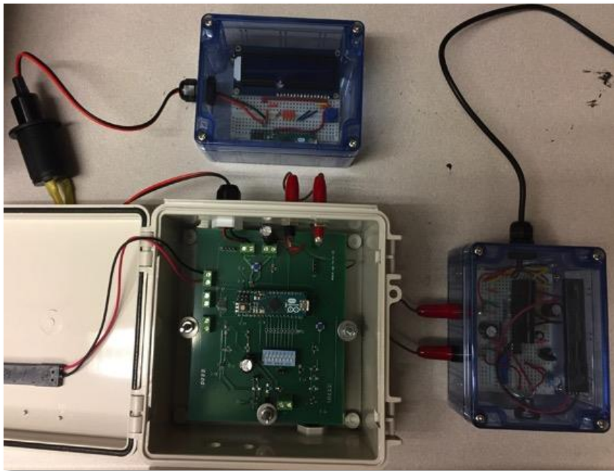
Figure 19: Wake-Up Radio Prototype
