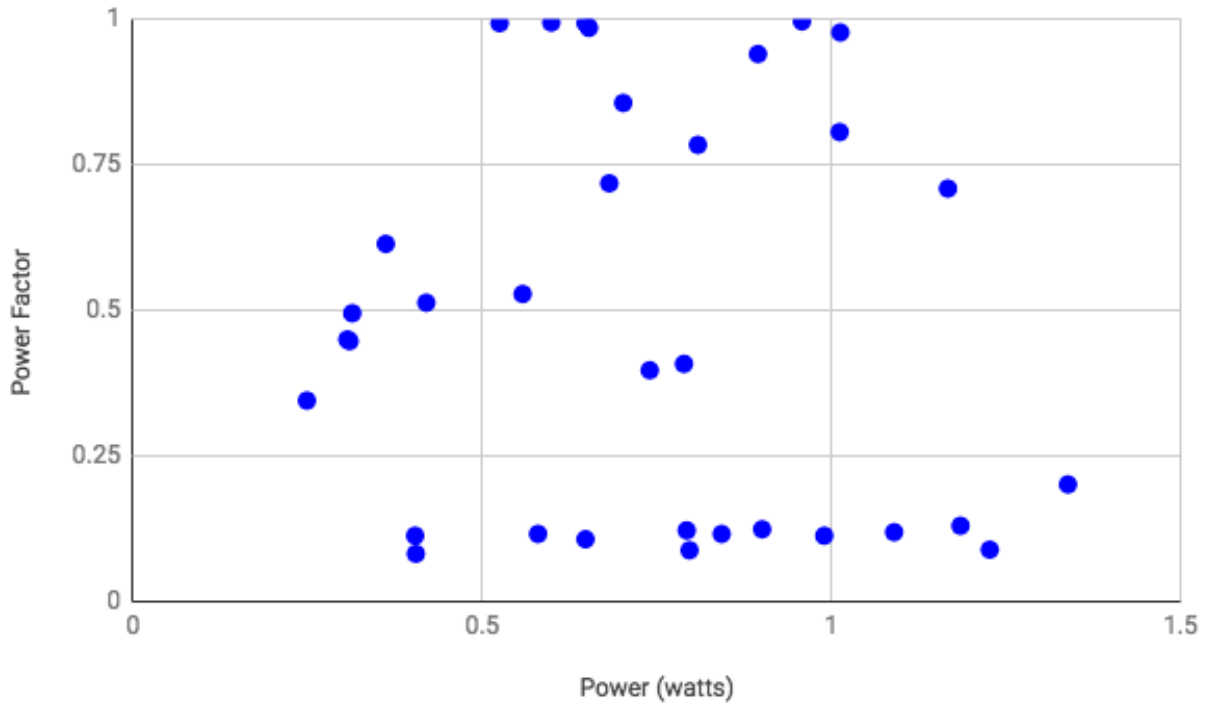
Figure 53: Plot of Power Factor with Respect to Power for All Tested Safety, Security, and Health Devices
