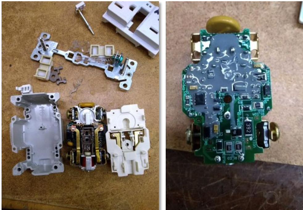
Figure 57: GFO38 GFCI Outlet Teardown
