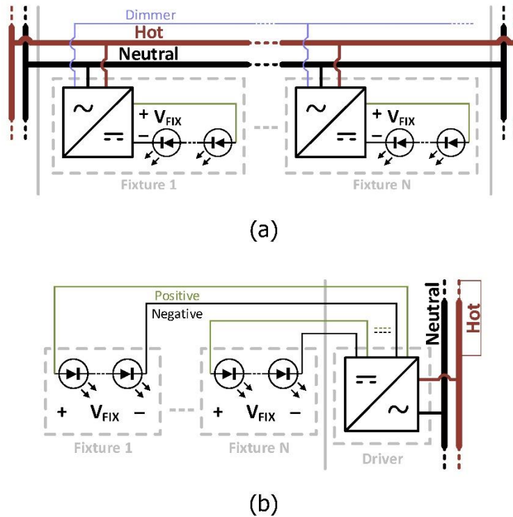
Figure 36: Direct Direct-Current Zone Light Modification
