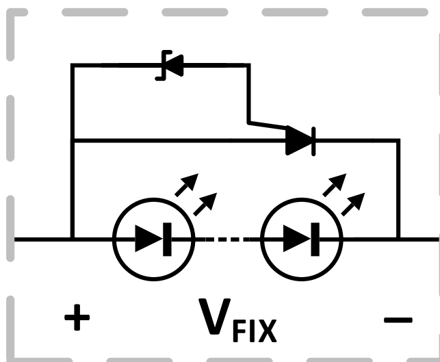
Figure 40: Fixture Bypass Circuit
