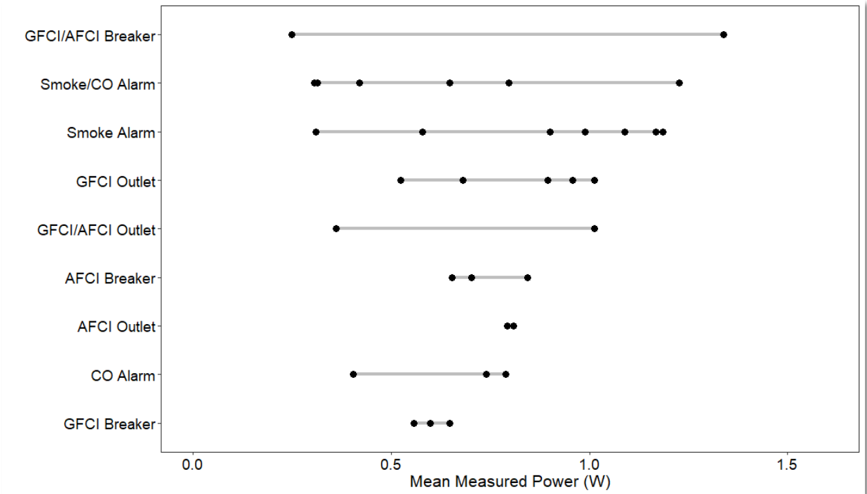
Figure 55: Measured Power Consumption of Safety, Security, and Health Devices
