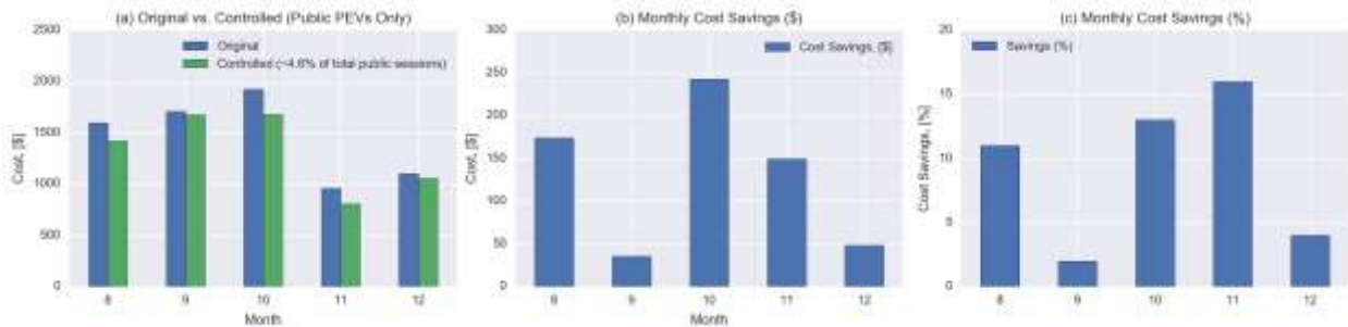
Figure 42: Cost Savings Considering Only Smart Charged Public Sessions at AICoPark Garage in August-December 2017
