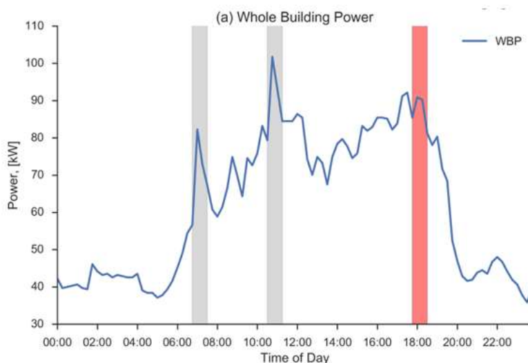
Figure 38: Whole Building Power with Highlighted Direct Current Fast Charging on October 3, 2017
