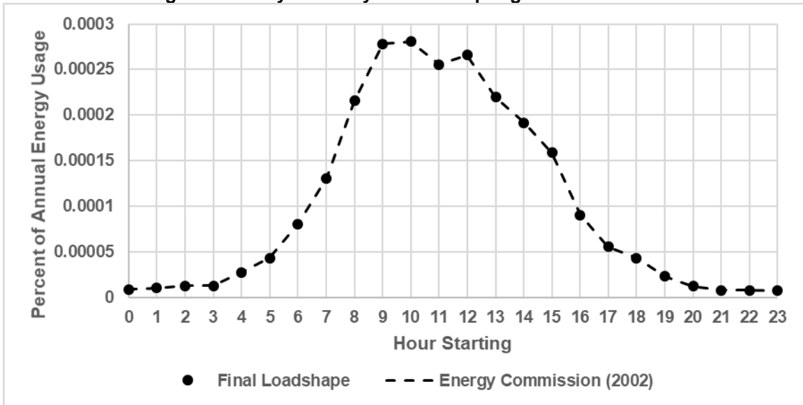
Figure 52: Daily Weekday Profile in Spring for Pool Heater
