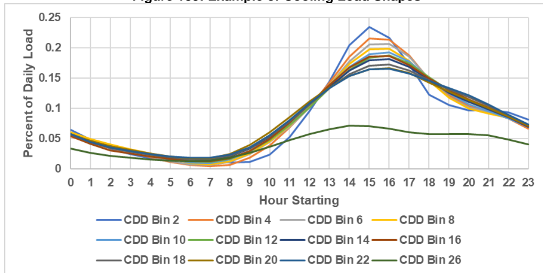
Figure 139: Example of Cooling Load Shapes
