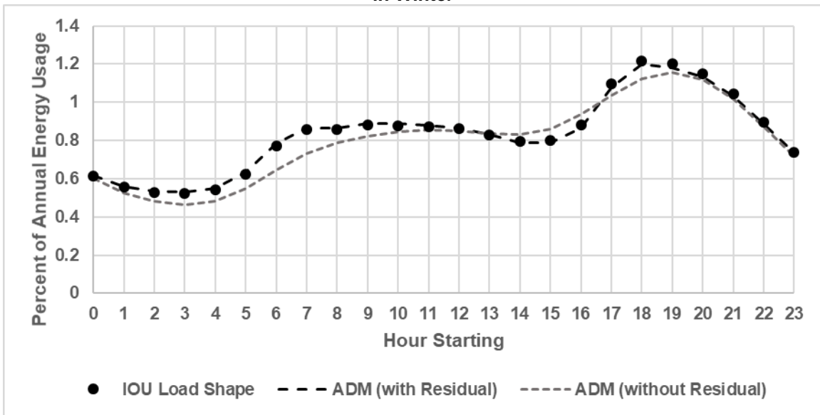
Figure 142: Comparison of the Average Daily Weekday Profile With and Without Residual in Winter
