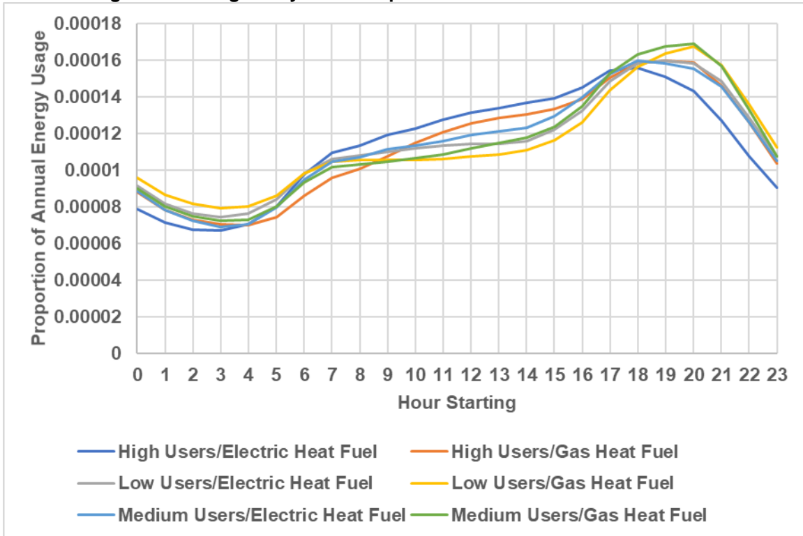
Figure 3: Average Daily Load Shape for Residential Customers in 2014
