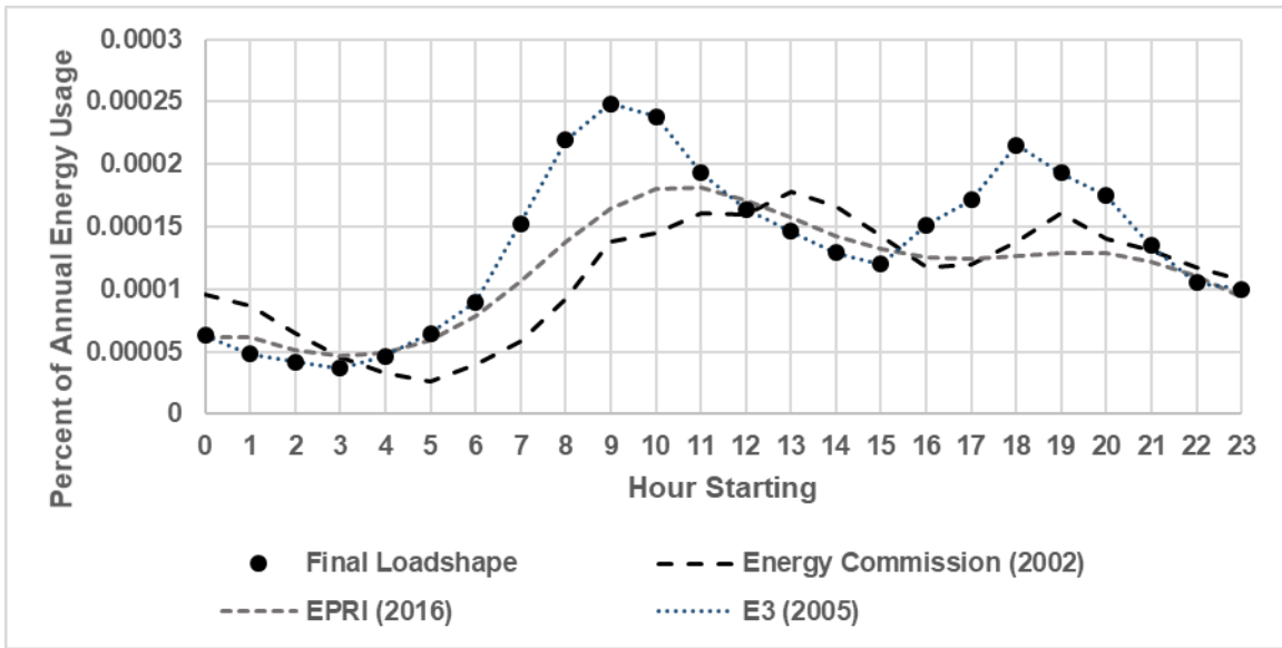
Figure 123: Comparison of the Average Daily Weekend Profile in Winter for Single-Family Water Heater
