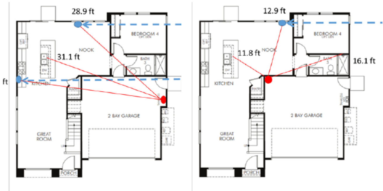
Figure 9-3: Water Heater Location
