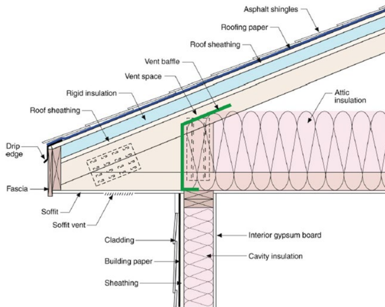
Figure 5-10: Attic with Above Deck Insulation
