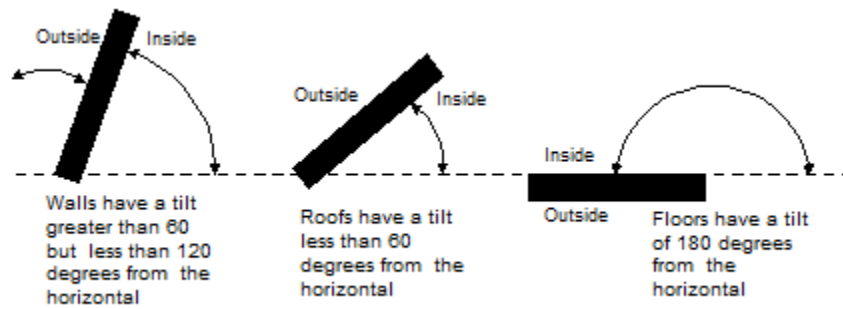
Figure 7-5: Surface Tilt
