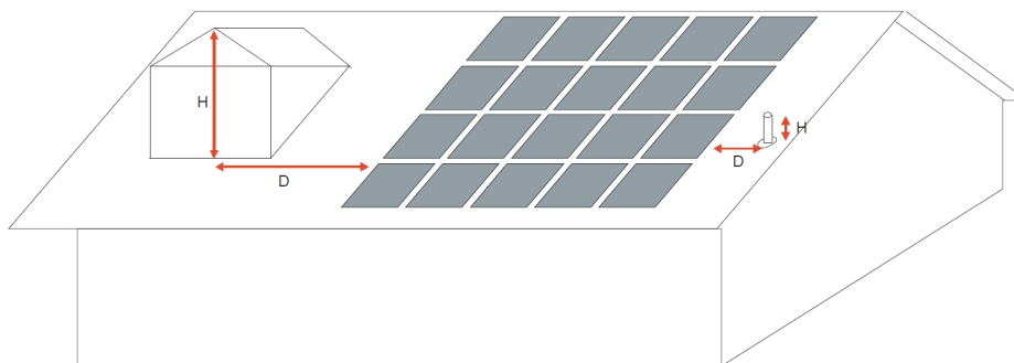
Figure 4-9: Minimal Shading Criterion
