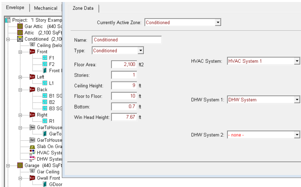
Figure 7-1: Conditioned Zone
