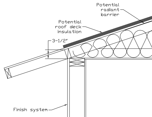
Figure 6-8: Section at Attic Edge with Standard Truss
