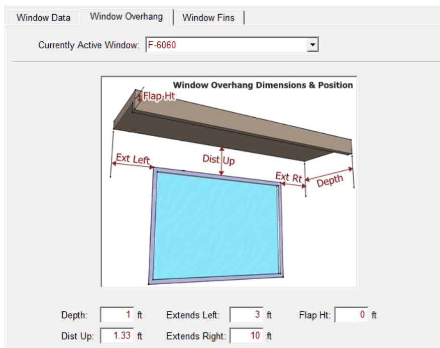
Figure 7-15: Overhang
