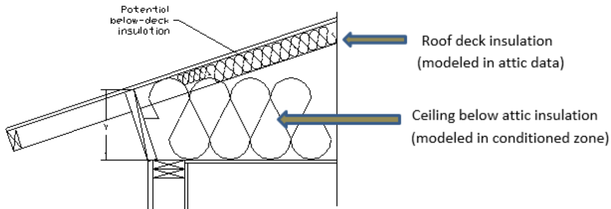
Figure 6-5. Attic insulation locations
