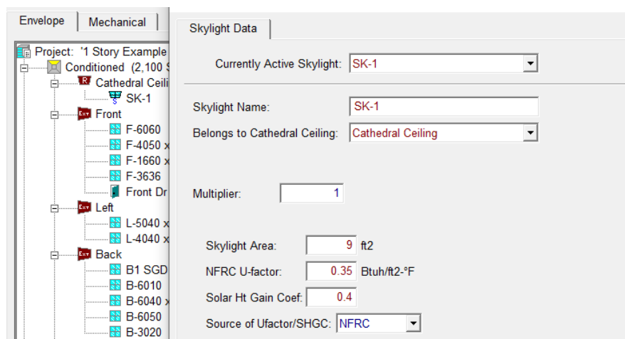
Figure 7-17: Skylight
