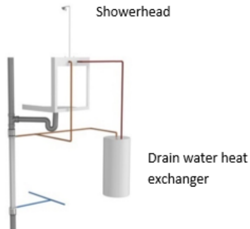
Figure 9-25: Drain Water Heat Recovery (Equal)
