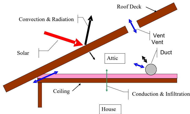
Figure 5-7: Attic Model Components
