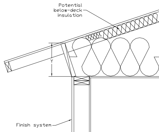
Figure 6-9: Section at Attic Edge with a Raised Heel Truss
