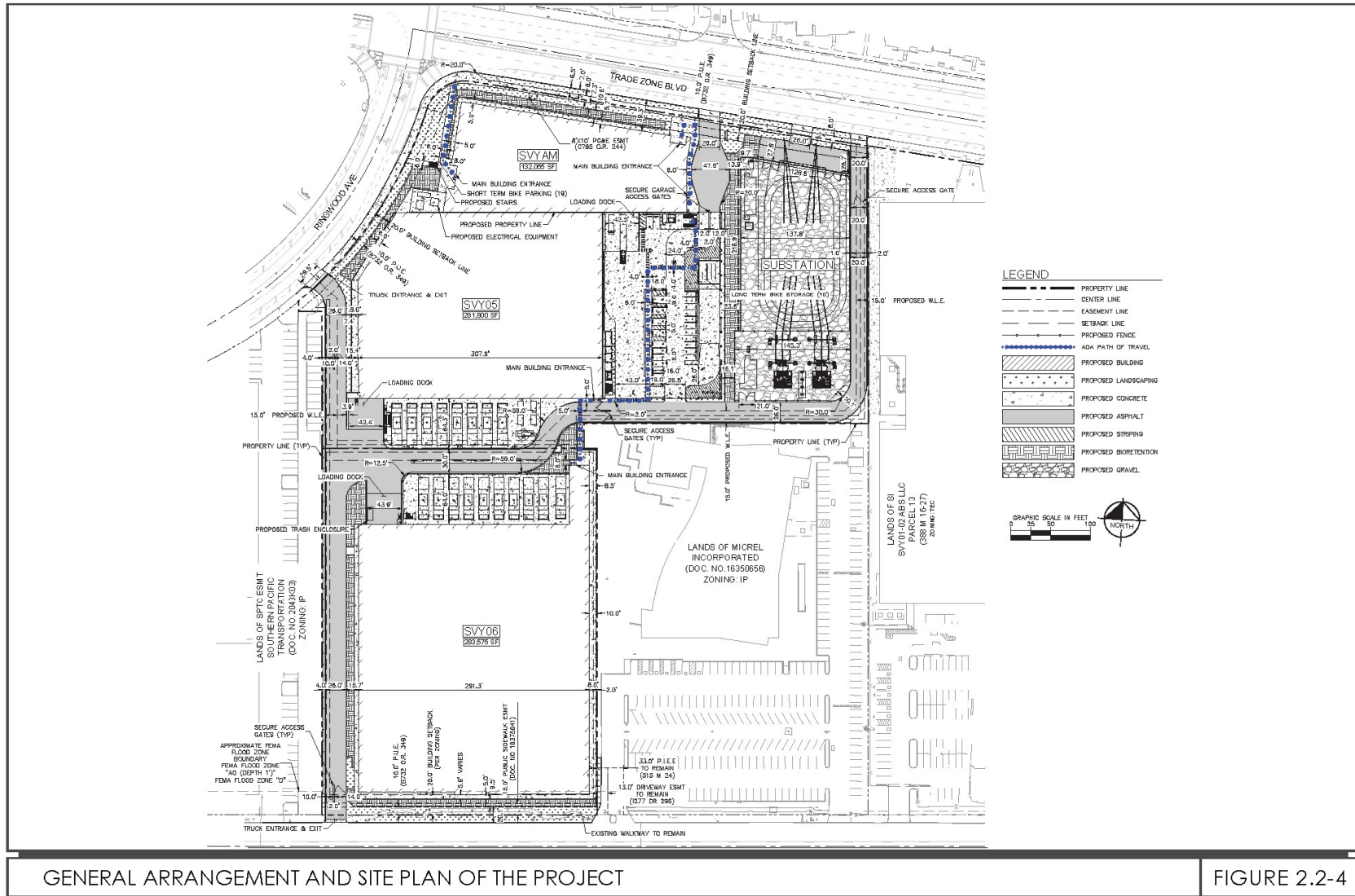
Figure 2.2-4 General Arrangement and Site Plan of the Project
