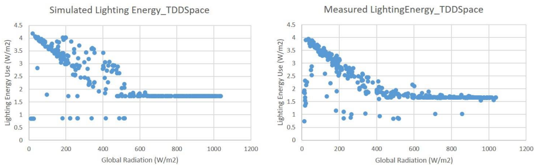
Figure C-2: Lighting Energy Use With Global Radiation - Simulated vs. Measured
