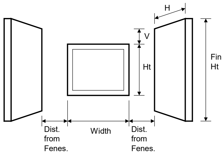
Figure 77: Sidefin Dimensions
