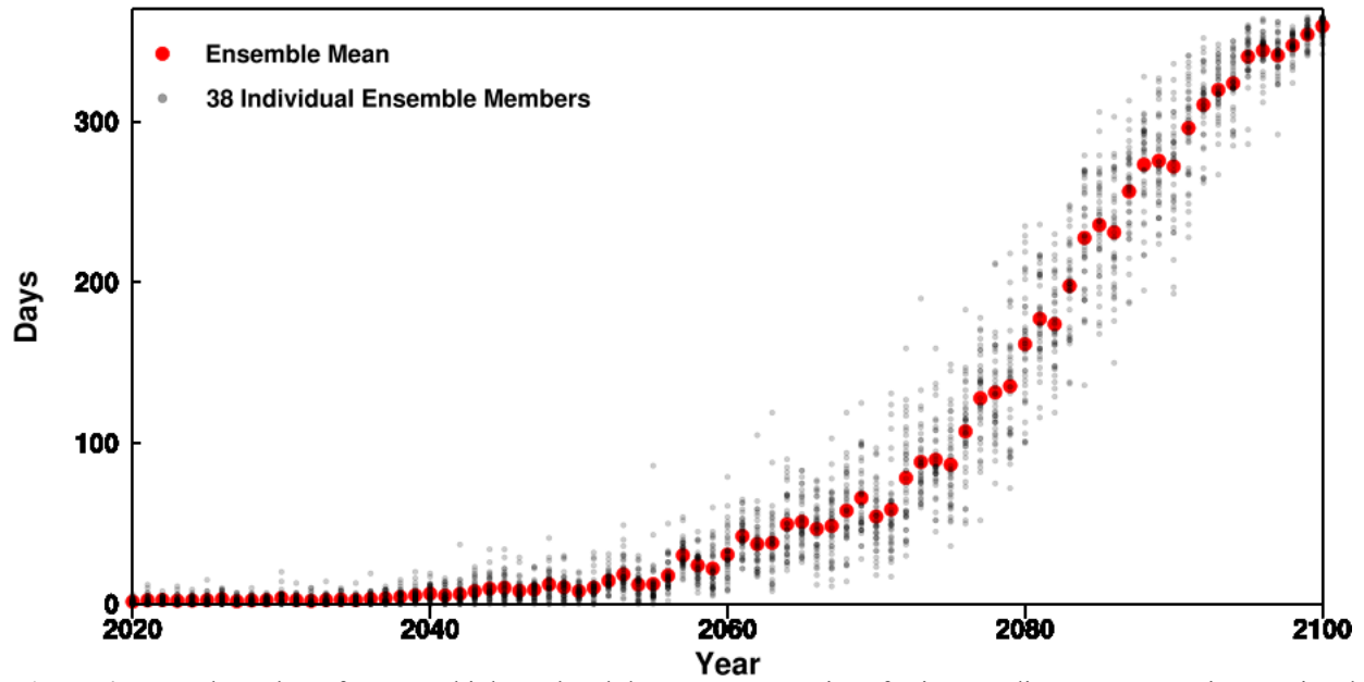
Figure 4. Annual number of extreme high sea level days at San Francisco for intermediate SLR scenario associated with SSP370 emission trajectory. Extreme days are defined as those with at least one hour above the historical (1950-2019) 99.99% hourly water level height at San Francisco for 38 individual model/ensemble members (gray dots) and the ensemble mean (red dots).
