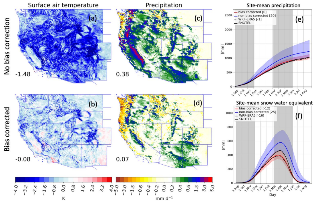
Figure 3. Relative to PRISM, ensemble-mean climatological (1981-2010) bias patterns in annual-mean (a,b) temperature and (c,d) precipitation, with 11-state-mean biases indicated in the lower-left of each subpanel. (e, f) time series of cumulative annual precipitation and snow water equivalent (SWE), respectively [mm], across 703 western U.S. SNOTEL sites. Shading denotes the range in w/BC (red) and no-BC (blue) experiments. Observations (black solid curve) and WRF-ERA5 (black dashed curve) are also presented.
