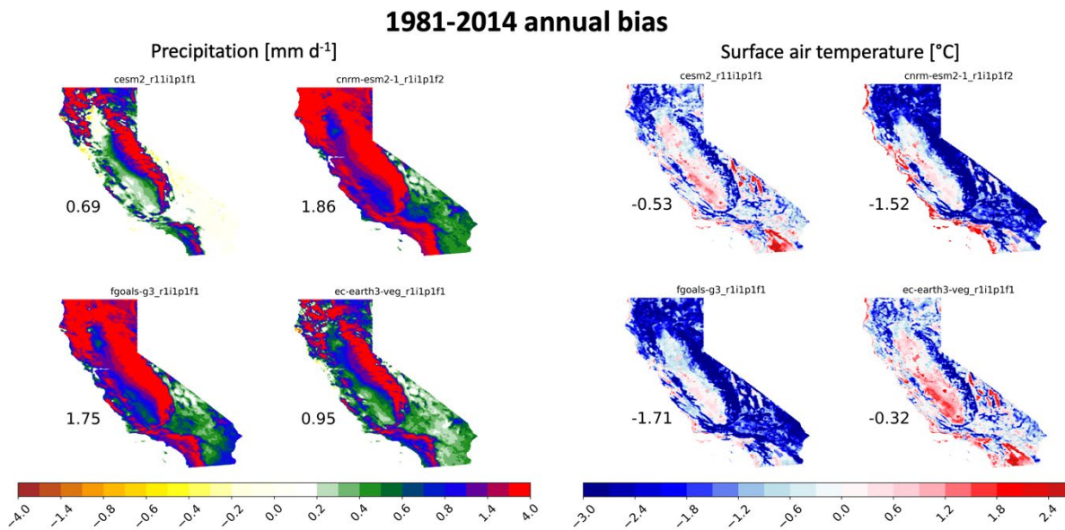
Figure 1. Historical-era (1981-2014) annual mean biases in (left) precipitation [ \text{mm d}^{-1} ] and (right) surface air temperature [ ^{\circ}\text{C} ] for the four original downscaled GCMs.
