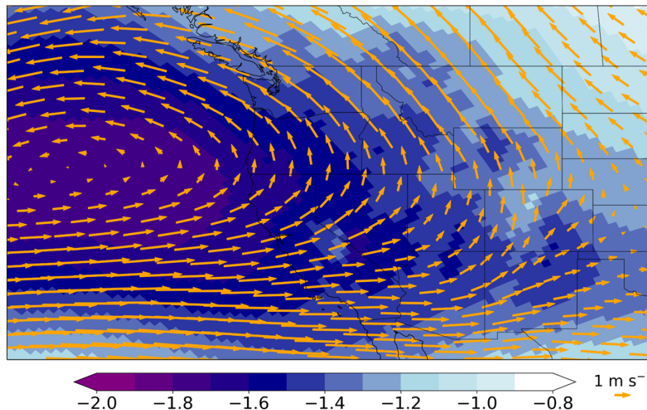
Figure 5. 1980-2014 biases in 9-GCM-mean 500 hPa temperature [°C] and 250 hPa horizontal winds [m s -1 ].
