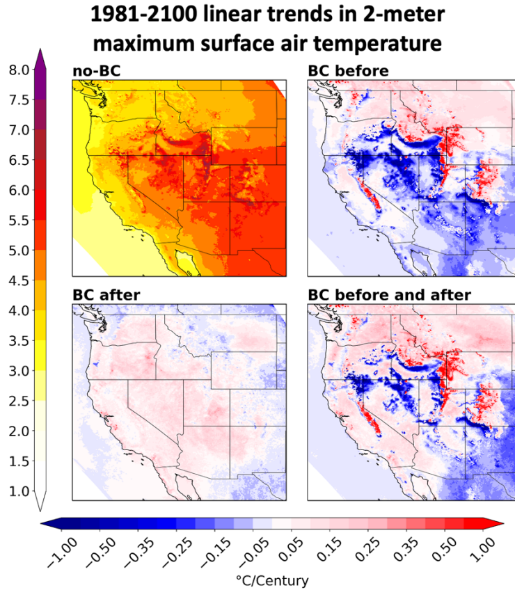
Figure 4. The upper-left panel shows downscaled 9-GCM-mean linear trends in springtime 2-meter maximum daily air temperature [ ^{\circ}\text{C}/\text{Century} ]. The upper-right panel depicts alterations in linear trends if BC is applied prior to downscaling for identical GCMs (subtracting the no-BC from the w/BC experiments). The bottom-left figure is the same as in the upper-right, but for linear trend alterations when BC is applied after downscaling only using PresRat. The bottom-right figure is the same as in the upper-right, but for linear trend alterations when BC is applied both before and after downscaling.
