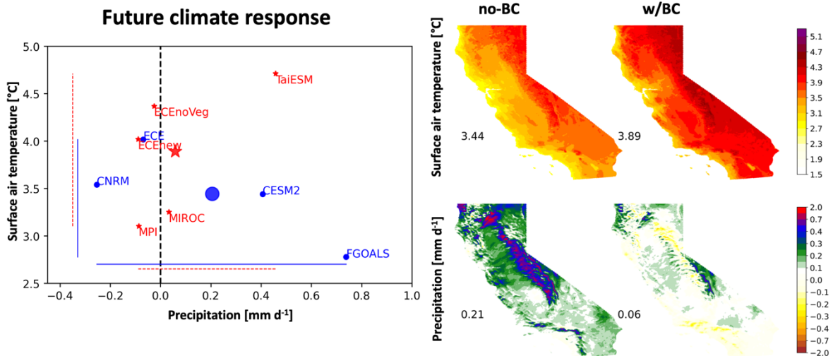
Figure 8. Future-era (2070-2099 mean) annual and California-mean changes in surface mean air temperature [ ^{\circ}\text{C} ] and precipitation [ \text{mm d}^{-1} ] relative to the 1981-2010 period. The left panel shows a scatter of future-era warming against future-era precipitation changes. Individual GCMs are shown as red stars (blue circles) for w/BC (no-BC) experiments with larger symbols indicating the ensemble mean changes. Red dashed (blue solid) horizontal lines showcase the precipitation spread. Vertical lines also denote spread but for temperature. Geographic figures on the right show the spatiality of (top) temperature and (bottom) precipitation changes for (left) no-BC and (right) w/BC experiments in their respective ensemble means. Numbers in the lower-left portion of each subpanel denote California-mean changes in either temperature [ ^{\circ}\text{C} ] or precipitation [ \text{mm d}^{-1} ].
