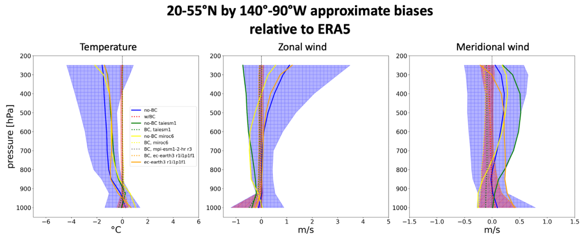
Figure 2. Regional-mean approximate downscaled GCM bias profiles from w/BC (dashed) and no-BC (solid) experiments across the Northeast Pacific and the western U.S. for (left) temperature [ ^{\circ}\text{C} ], (center) zonal wind [ \text{m s}^{-1} ], and (right) meridional wind [ \text{m s}^{-1} ]. Here, these are approximate biases because the reference data product used here is ERA5-WRF (see LOCA Version 2 – Training Data Adoption Justification Memo). Since we are using spectral nudging in the 45-km WRF experiments, these fields are approximately conserved in downscaling across large spatial scales. Here, no-BC and w/BC are constructed using an identical 11-GCM mean with their spreads given by blue and red shading, respectively. We also include individual curves for new GCMs reported to CEC (all bias corrected; dashed curves) and where possible, the no-BC pair (not reported to CEC).
