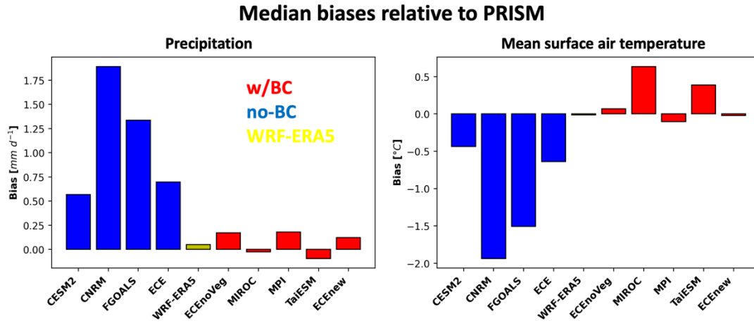
Figure 7. California-mean historical biases in median (left) precipitation [ \text{mm d}^{-1} ] and (right) daily mean surface air temperature [ ^{\circ}\text{C} ] from individual GCMs within no-BC (blue) and w/BC (red) simulations. WRF-ERA5 is provided for reference.
