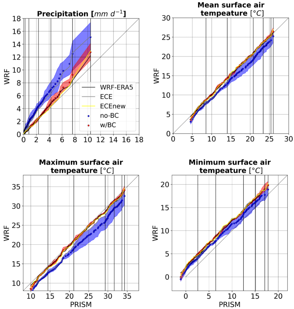
Figure 6. California-mean historical-era WRF-simulated variables scattered against reference data from PRISM by quantile for (upper-left) precipitation [ \text{mm d}^{-1} ], mean surface air temperature [ ^{\circ}\text{C} ], maximum surface air temperature [ ^{\circ}\text{C} ], and minimum surface air temperature [ ^{\circ}\text{C} ]. GCM means of the original 4 (no-BC) simulations comprise the blue scatter, while GCM means from the new 5 (w/BC) simulations are depicted by the red scatter. Red (blue) shading denotes the w/BC (no-BC) experimental spread, and the WRF-ERA5 is depicted by the black solid line. EC-Earth3-Veg is the only experiment that was duplicated in the w/BC and no-BC runs and is depicted by the light yellow and gray curves, respectively. Vertical bolded lines indicate the 25 th , 50 th (median), 75 th , 90 th , 99 th , and 99.9 th percentile values from PRISM.
