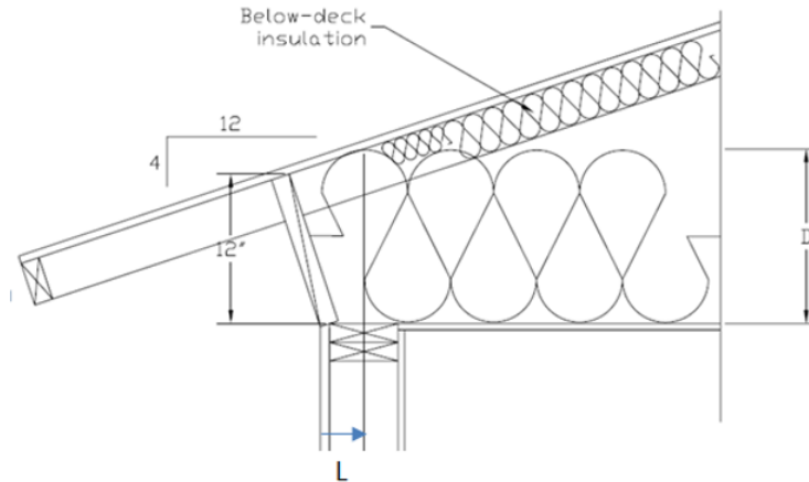
Figure 27: Raised-Heel Geometry
