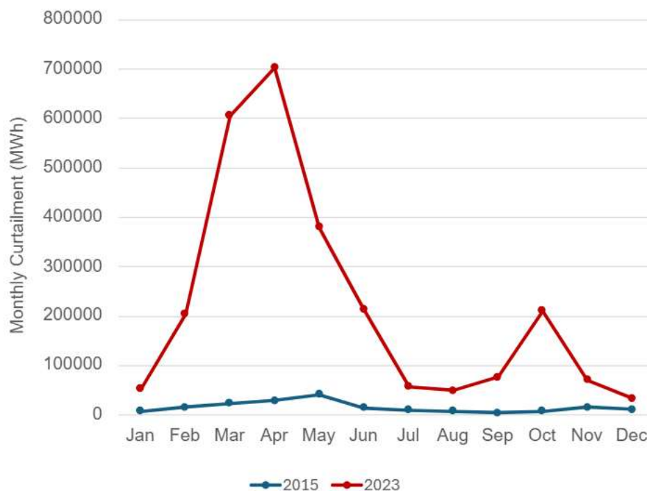
Figure 10: California ISO Renewable Curtailments
