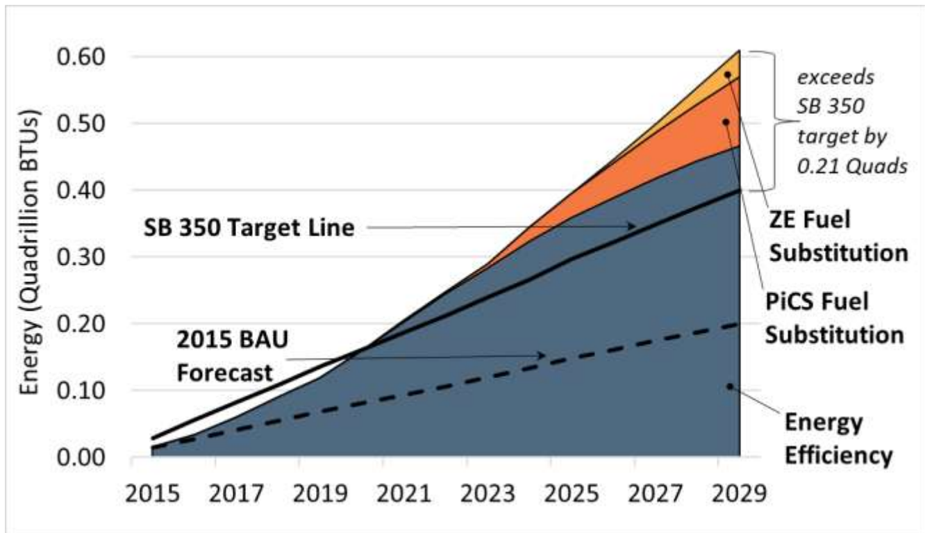
Figure 16: SB 350 Scenario Two Combined Energy Compared to the Doubling Target
