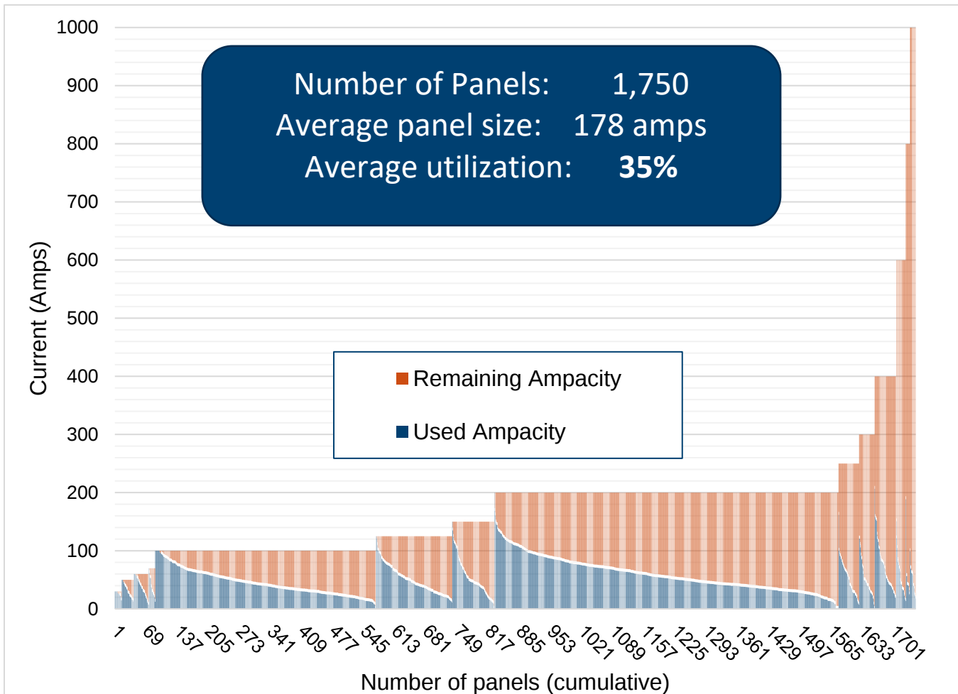
Figure 8: Electric Panel Size and Used Capacity (amps)
